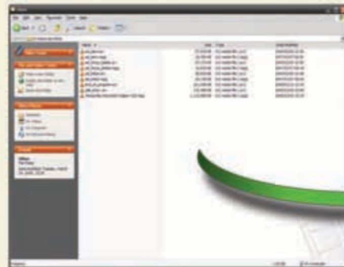
Windows Explorer
